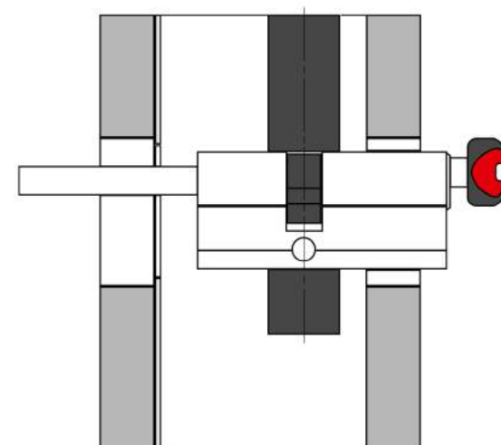
Figure 30 – Setting the cylinder on the axis
